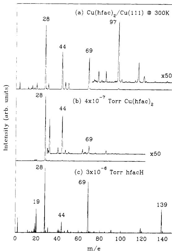
Figure 9. (a) IDMS spectrum of the species desorbing from a Cu(111) surface exposed to 20 L of Cu(hfac) 2 at 300 K. Data were obtained between 350 and 650 K at a heating rate of 2 K/s. Similar spectra have been recorded for Cu(hfac)(vtms) and hfacH. 12 Mass spectra of gas-phase Cu(hfac) 2 and hfacH recorded with the same quadrupole settings are shown in traces b and c, respectively.
