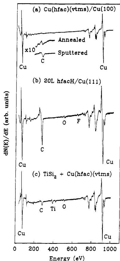
Figure 13. Auger electron spectrum of (a) a clean Cu(100) surface exposed to 20 L of Cu(hfac)(vtms) at 300 K and flashed to 600 K. Only trace carbon impurities are observed. In the lower trace the experiments were repeated, except the surface was sputtered with \sim 5 \mu\text{A} of 1 keV \text{Ne}^+ ions at room temperature for 5 min without annealing to create a significant number of surface defects. In this latter case, slightly more carbon is observed. In b the Cu(111) surface was exposed to 10 cycles of 20 L of hfacH at 300 K and then heated to 650 K. Significantly more carbon is seen in this case. Trace c shows that a thin film of relatively pure copper can be grown from Cu(hfac)(vtms) under high vacuum conditions ( 1 \times 10^{-5} Torr, 500 K, 10 min) on a TiSi 2 substrate.
