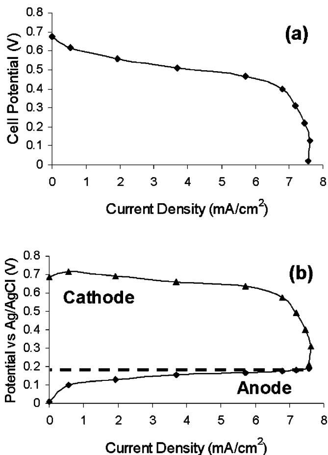
Figure 2. Reference electrode experiment to isolate cathode and anode performance in an LF-FC. Polarization curves for (a) the overall cell performance; and (b) the individual anode and cathode. Fuel: 1.0 M methanol in 0.5 M H_2SO_4 . Oxidant: oxygen-saturated 0.5 M H_2SO_4 . Anode and cathode catalysts are Pt:Ru 50:50 alloy unsupported nanoparticles and Pt black unsupported nanoparticles, respectively, at a loading of 2.0 mg/cm 2 . Flow rate: 0.3 ml/min per inlet channel. Channel length: 2.9 cm, width: 1.0 mm, height: 1 mm. Re = 6.7 . Experimental error \pm 3\% .
