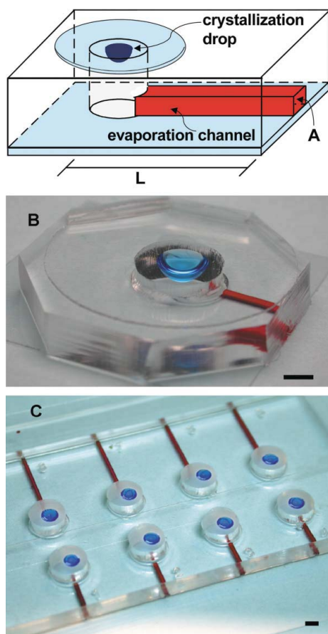
Figure 2 (A) Schematic of the platform: a compartment with a drop containing protein and precipitant, connected to the atmosphere through an evaporation channel of length L and cross-sectional area A . (B) Optical micrograph of the platform: red and blue ink is used to visualize the channel and the drop, respectively. (C) Optical micrograph of multiple wells cast in a single polymer slab. Scale bar: 2 mm
