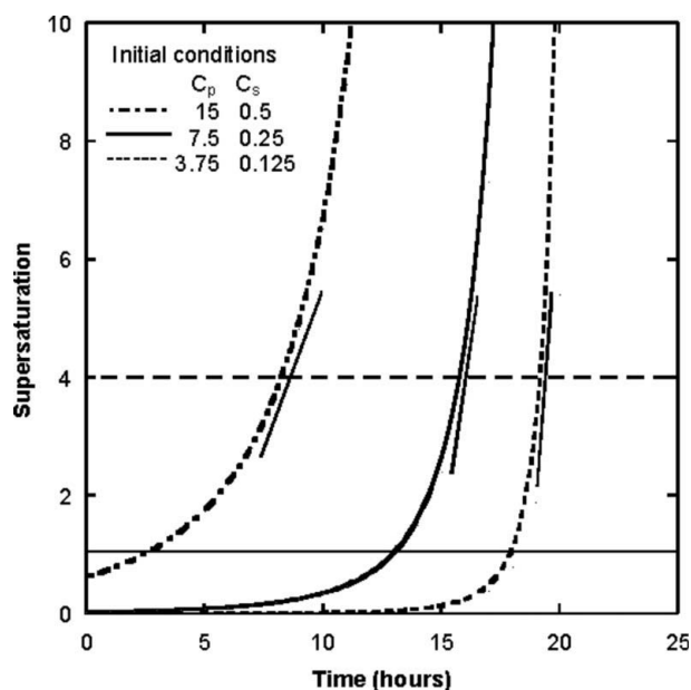
Figure 5 Supersaturation as a function of time for the crystallization of lysozyme. The lines are for a 10 \mu\text{l} drop and an evaporation rate J of 0.42 \mu\text{l h}^{-1} . These experiments are at different initial conditions but at a constant C_p/C_s ratio of 30 \text{ g mol}^{-1} . The initial conditions correspond to those of the lysozyme experiments in Figs. 3A–3C. The tangential lines indicate the rate of change of supersaturation, while the drop entering the labile region at S = 4 (see text) is indicated by the dashed horizontal line. The solid horizontal line at S = 1 is the solubility boundary.
