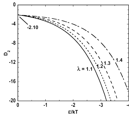
Figure 1. Plots of D_2 as a function of \epsilon/kT for different \lambda .
