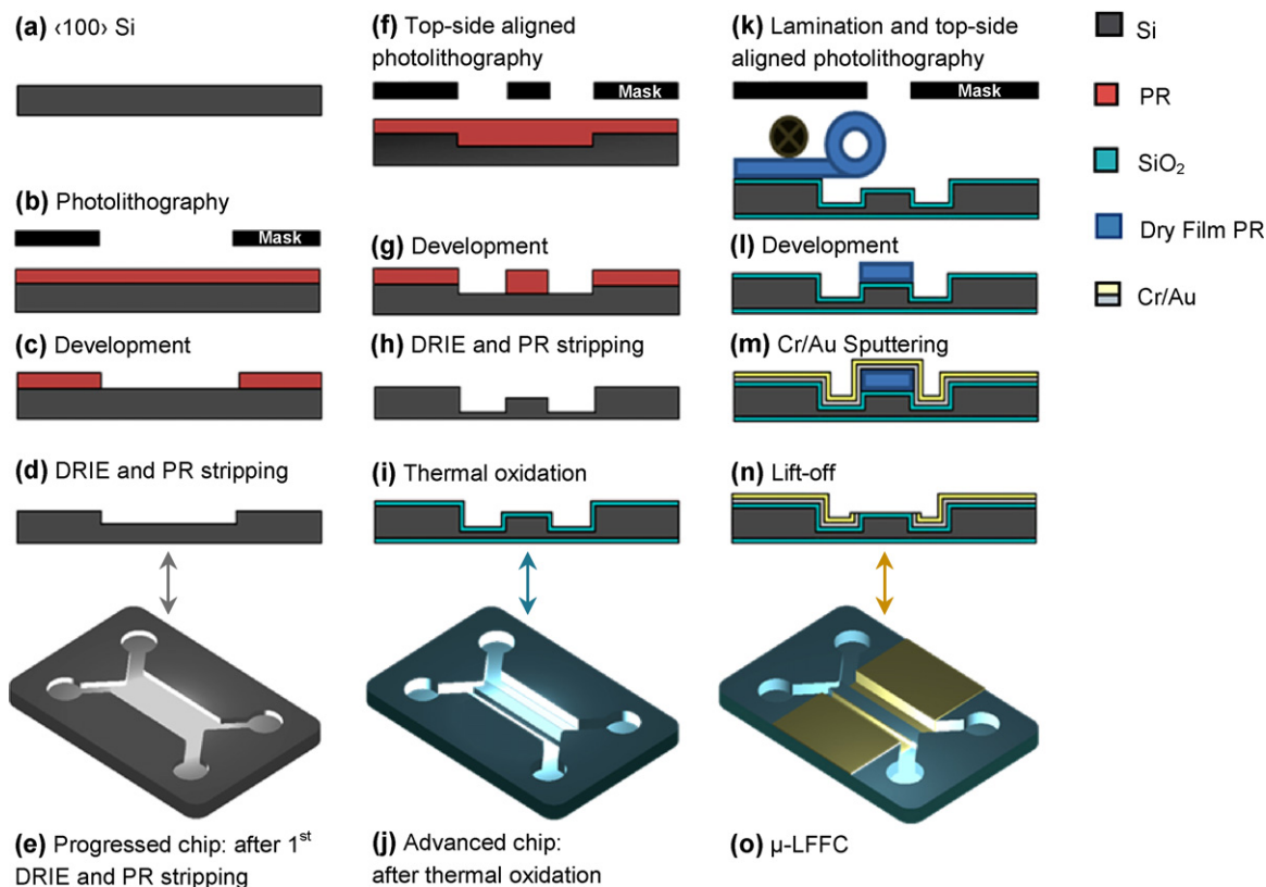
Fig. 5. \mu LFFC fabrication flow scheme: (a)–(e) 10\ \mu\text{m} DRIE, (f)–(j) 50 – 75\ \mu\text{m} DRIE (microchannels and feedholes) followed by Si thermal oxidation ( \text{SiO}_2 ) and (k)–(o) integration of the Cr/Au current collectors.
