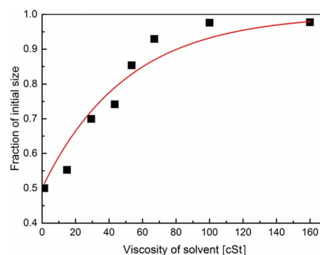
Figure 4. Effect of viscosity on fragmentation of potassium chloride. A slurry containing 0.2 wt% potassium chloride in a dodecane-silicon oil mixture was sonicated using a titanium horn ( 10\text{ W cm}^{-2} and 20 kHz). The solid line is an exponential fit.
