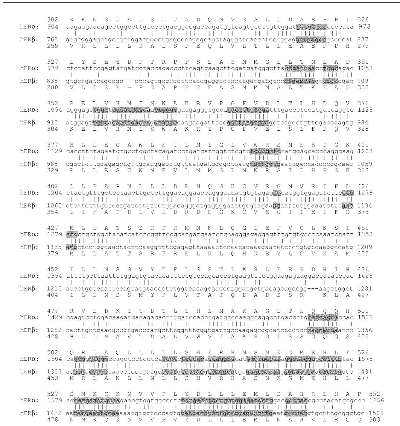
Figure 3. The results of DNA shuffling from cDNAs of the ER \alpha and ER \beta ligand binding domains. DNA sequence alignment between the ER \alpha and ER \beta ligand binding domains is shown based on their amino acid sequence alignment. The sites of crossover are highlighted.
