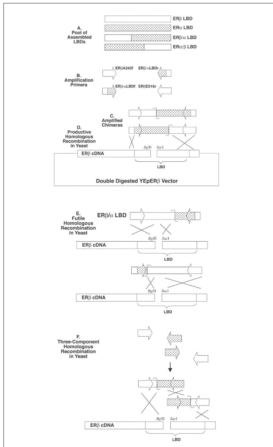
Figure 1. DNA shuffling /homologous recombination system. (A) The assembled ER ligand binding domain (LBD) pool after DNA shuffling. The full-length assembled ligand binding domains are mostly non-chimeric, either ER \alpha or ER \beta , with a small portion of chimeric ER \alpha / \beta and ER \beta / \alpha . (B) Use of primer pairs ER \alpha A242f and ER \beta / \alpha LBDr or ER \beta / \alpha LBDf and ER \beta E516r in the PCR amplification from assembled ligand binding domain products. (C) Only chimeric sequences can be successfully amplified using the above primer pairs. (D) In vivo homologous recombination between the chimeric ligand binding domain sequences and digested YEpER \beta vector, based on the identical sequences at both ends of the ligand binding domains and sequences in the vector, as indicated by the crossing lines. (E) In vivo homologous recombination within the ligand binding domain sequence results in wild-type products. (F) Two pairs of primers used for PCR generate two partial but overlapping chimeric ligand binding domain fragments; those fragments undergo homologous recombination with a linearized vector to form an ER expression vector carrying two crossovers in the ligand binding domain.
