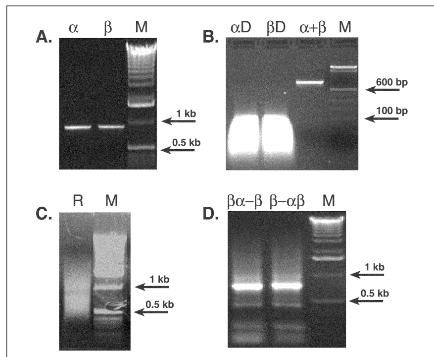
Figure 2. DNA shuffling between ER \alpha and ER \beta ligand binding domains. (A) The ligand binding domain cDNAs from ER \alpha and ER \beta were amplified with primer pairs ER \alpha A289f and ER \alpha S566r (lane \alpha ) or ER \beta A242f and ER \beta E516r (lane \beta ), respectively. Lane M, 1-kb DNA ladder (Invitrogen). (B) The partial DNase I digestion of cDNAs of ER \alpha ligand binding domain (lane \alpha D) and ER \beta LBD (lane \beta D). Their original size is shown in Lane \alpha + \beta for comparison. Lane M, 100-bp DNA ladder (Invitrogen). (C) Lane R, the products after assembly; lane M, 1-kb DNA ladder (Invitrogen). (D) The amplifications of chimeric products from the assembled products. Primers ER \beta / \alpha LBDf and ER \beta E516r were used in the PCR to amplify chimeric ligand binding domains that have N-terminal sequences from ER \alpha and C-terminal sequences from ER \beta (lane \beta \alpha - \beta ). Primers ER \beta A242f and ER \beta / \alpha LBDr were used in the PCR to amplify chimeric ligand binding domains that have N-terminal sequences from ER \beta and C-terminal sequences from ER \alpha (lane \beta - \alpha \beta ). Lane M, 1-kb DNA ladder (Invitrogen).
