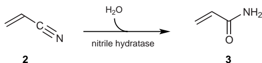
Scheme I. Example of an enzyme assisted synthesis.
