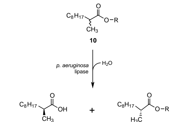
Scheme IV. Enantioselective hydrolysis of 2-methyldecanoate, 10 .
