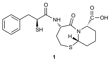
Figure 1. Omapatrilat, a vasopeptidase inhibitor.
