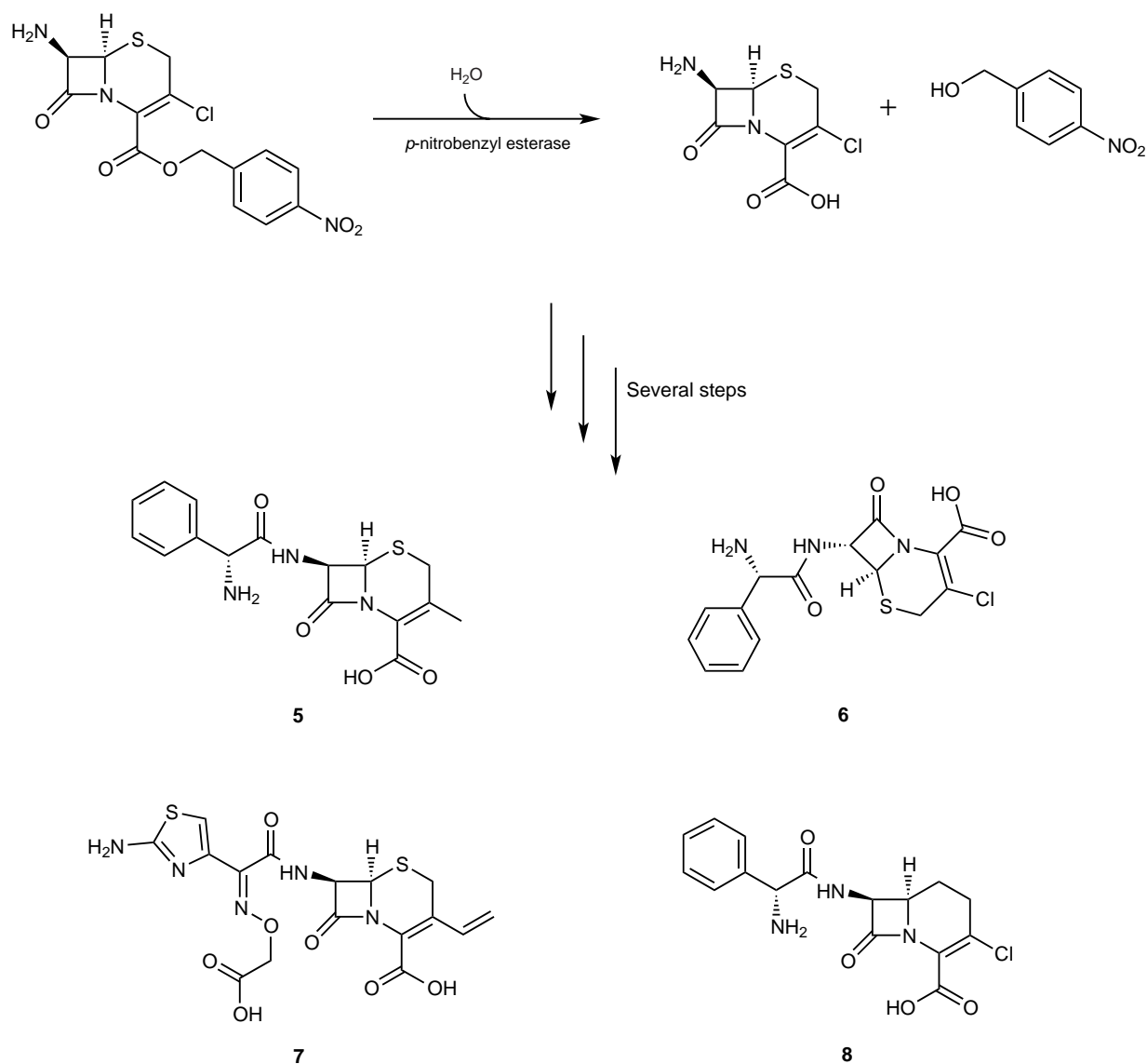
Scheme II. Use of a modified enzyme in a nonaqueous solvent to produce antibiotics, 5-8 .
