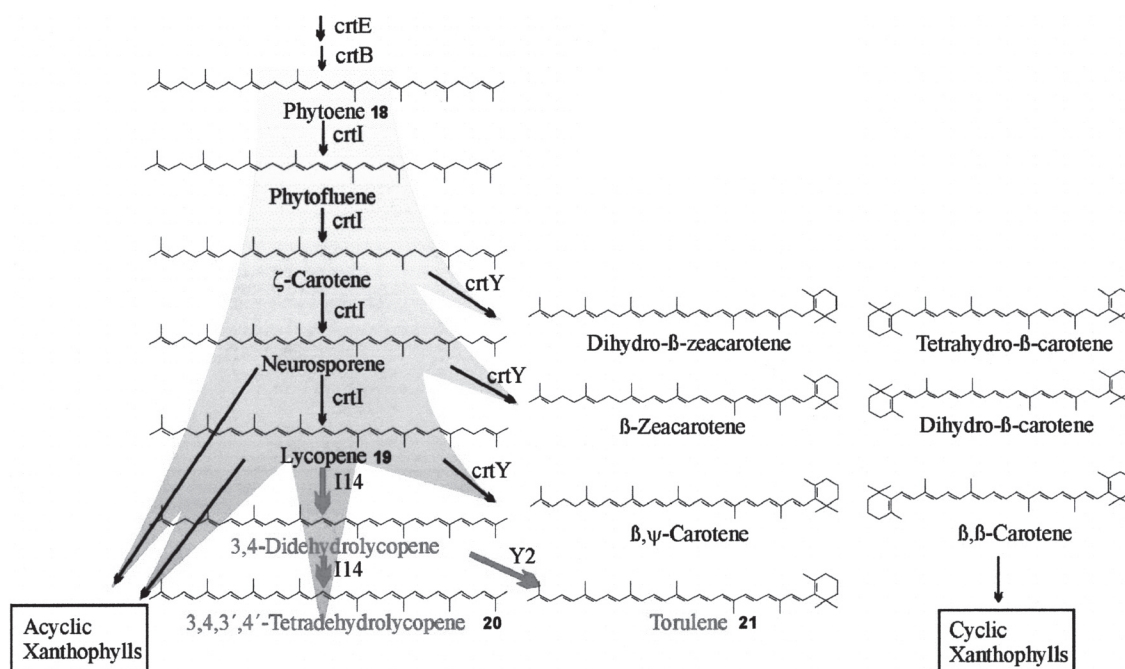
Figure 7. Molecular breeding of novel carotenoid biosynthetic pathways. Thick arrows indicate how the central desaturation pathway has been extended to obtain the fully conjugated 3,4,3',4'-tetrahydrolycopene and subsequent branching of this pathway for the synthesis of the novel cyclic carotenoid torulene in E. coli . The compounds listed on the left-hand side are acyclic carotenoid compounds while those listed in the middle and on the right-hand side are cyclic carotenoid compounds. (This figure was adapted from ref 31 with permission.)
