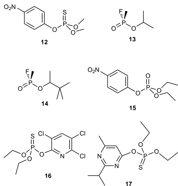
Figure 6. Examples of neurotoxic organophosphates used as pesticides.
