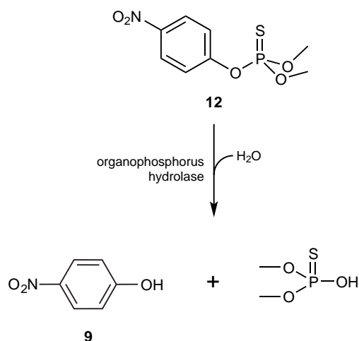
Scheme VI. Improved degradation of pesticide 12 by a modified enzyme.
