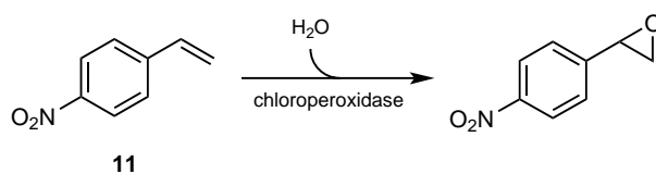
Scheme V. Epoxidation reaction using a modified enzyme.
