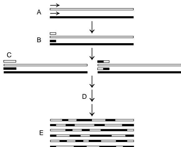
Figure 5. Schematic representation of the StEP in vitro recombination method. Only one primer and single strands from two parental genes (templates) are shown. (A) Denatured template genes are primed with one defined primer. (B) Short fragments are produced by brief polymerase-catalyzed primer extension. (C) Through another cycle of StEP, fragments randomly prime the templates (template switching) and extended further. (D) This process is repeated until full-length genes are produced. (E) Full-length genes are purified and (optionally) amplified in a PCR reaction with external primers. (Figure adapted from ref 32 with permission.)
