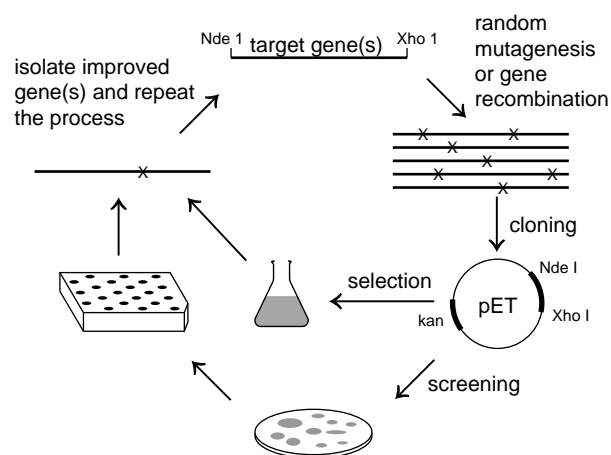
Figure 3. Schematic representation of directed evolution. As with Darwinian natural evolution, genetic diversity is introduced into a target gene through random mutagenesis or gene recombination. Functionally improved mutants are first identified by a selection or high throughput screening method and then used as the parents for next round of evolution. The process will be repeated until the goal is achieved.
