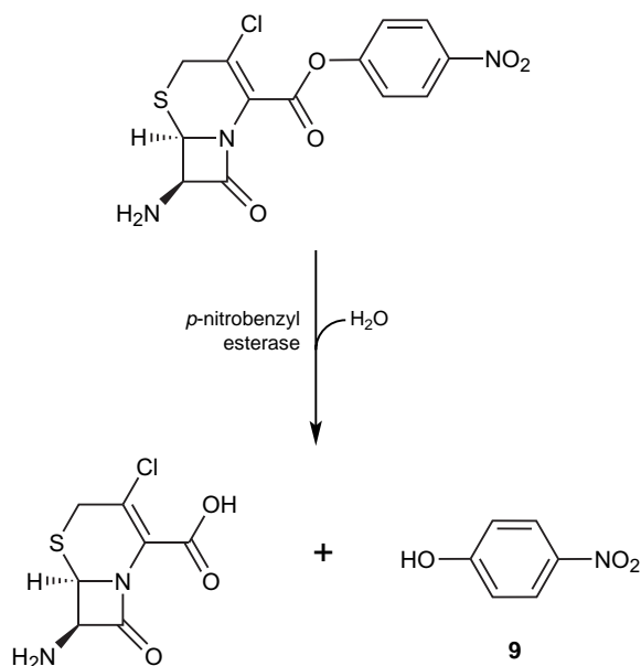
Scheme III. Reaction for the colorimetric screening assay.
